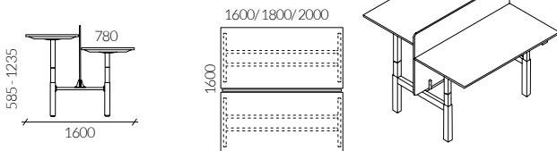
Lano-E 300 F Bench
