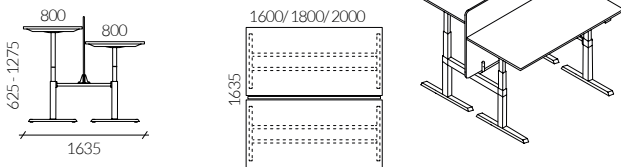
Lano-E 300 T Bench
